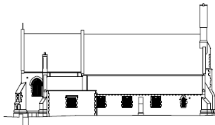
Existing North Elevation 1:100 @A1
