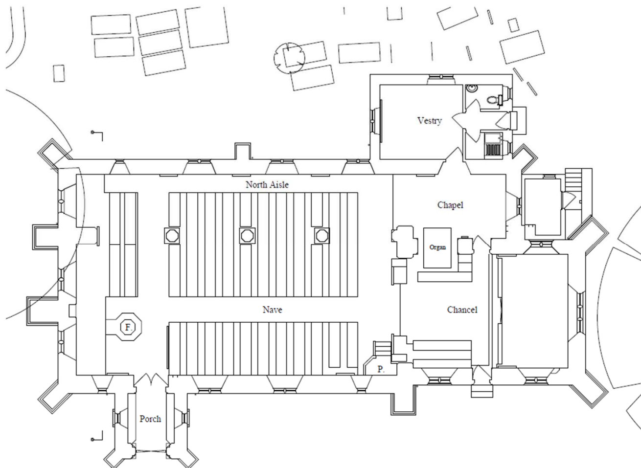
EXISTING PLAN
